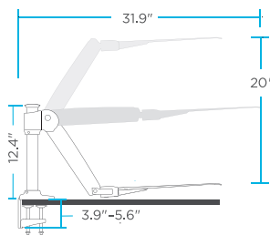
Profile View
